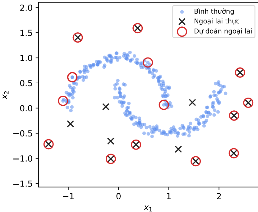
One-Class SVM — RBF, \nu=0.048
